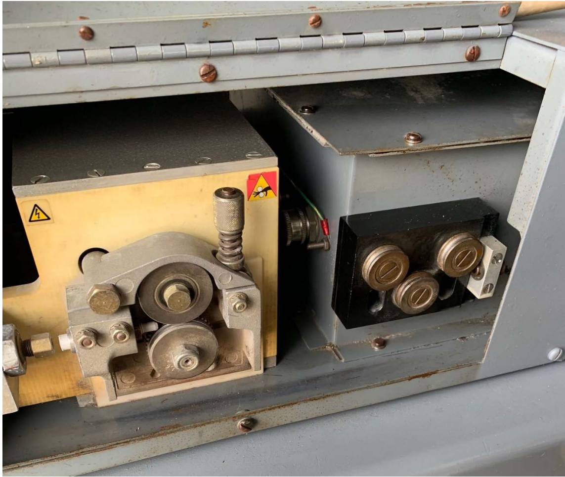
Left and right straightener/drive roll units
