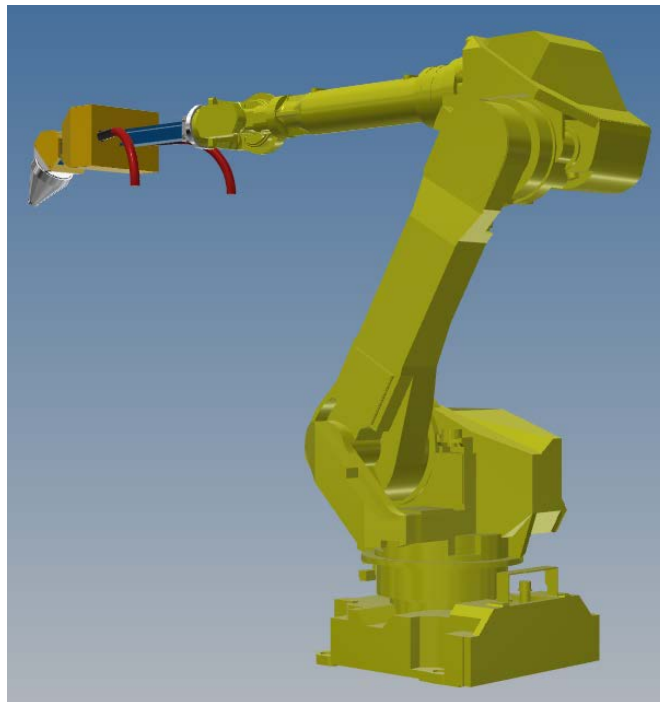
Pivot Arc Spray added as full axis on robot.
